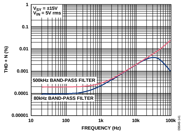
Figure 46. THD + N vs. Frequency, V_{SY} = \pm 15\text{ V}
