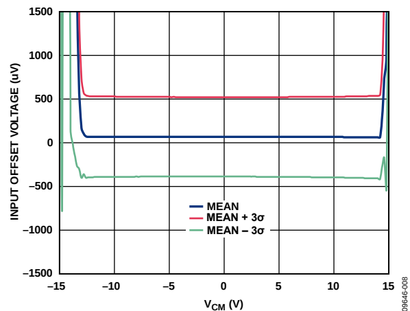
Figure 13. Input Offset Voltage vs. Input Common-Mode Voltage ( V_{CM} ), V_{SV} = \pm 15\text{ V} , R_L = \infty
