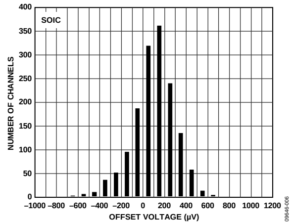
Figure 11. Input Offset Voltage Distribution, V_{SV} = \pm 15\text{ V}
