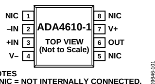
Figure 2. ADA4610-1 Pin Configuration, 8-Lead SOIC_N (R Suffix)
