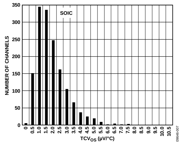
Figure 12. TCV_{OS} Distribution, V_{SV} = \pm 15\text{ V}
