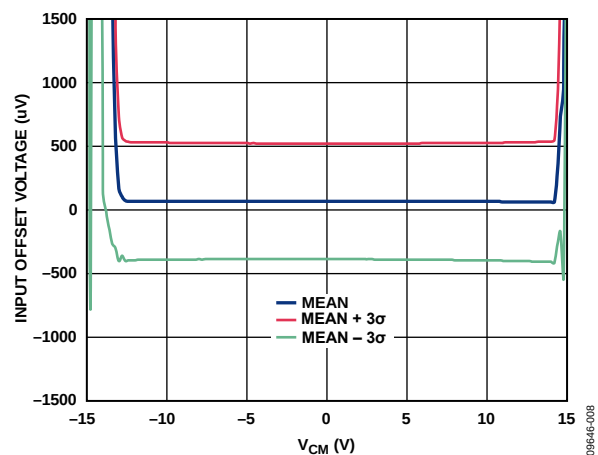
Figure 13. Input Offset Voltage vs. Input Common-Mode Voltage ( V_{CM} ), V_{SV} = \pm 15\text{ V} , R_L = \infty
