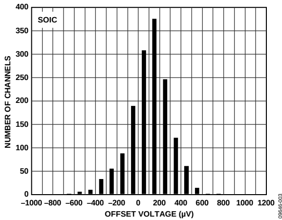
Figure 8. Input Offset Voltage Distribution, V_{SV} = \pm 5\text{ V}
