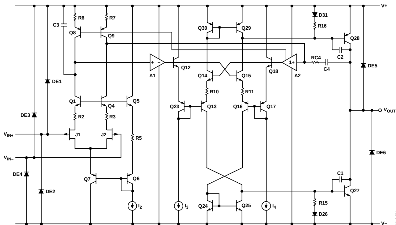
Figure 56. Simplified Schematic
