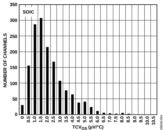
Figure 9. Input Offset Voltage Drift ( TCV_{OS} ) Distribution, V_{SV} = \pm 5\text{ V}
