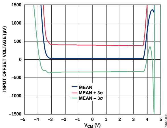
Figure 10. Input Offset Voltage vs. Common-Mode Input Voltage ( V_{CM} ), V_{SV} = \pm 5\text{ V} , R_L = \infty
