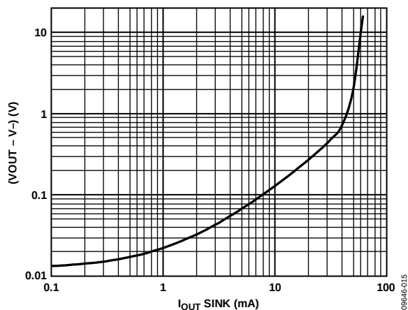
Figure 21. Dropout Voltage ( V_{OUT} - V^- ) vs. I_{OUT} Sink, V_{SY} = \pm 5\text{ V}
