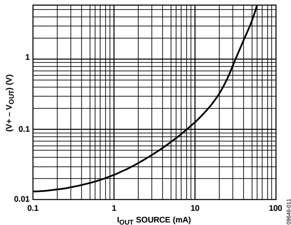
Figure 20. Dropout Voltage ( V^+ - V_{OUT} ) vs. I_{OUT} Source, V_{SY} = \pm 5\text{ V}
