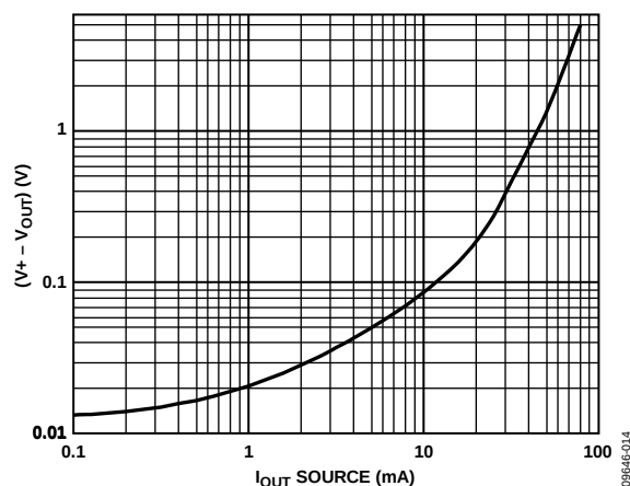
Figure 23. Dropout Voltage ( V^+ - V_{OUT} ) vs. I_{OUT} Source, V_{SY} = \pm 15\text{ V}
