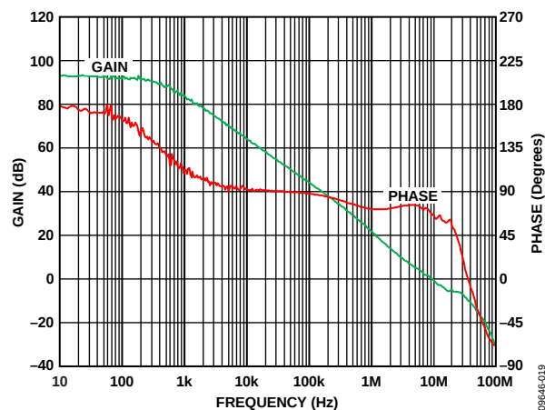
Figure 25. Open-Loop Gain and Phase vs. Frequency, V_{SY} = \pm 15\text{ V} , R_L = 2\text{ k}\Omega , V_{IN} = 5\text{ mV}
