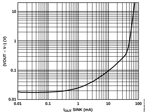
Figure 24. Dropout Voltage ( V_{OUT} - V^- ) vs. I_{OUT} Sink, V_{SY} = \pm 15\text{ V}
