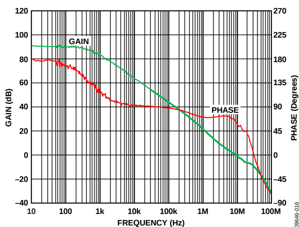
Figure 22. Open-Loop Gain and Phase vs. Frequency, V_{SY} = \pm 5\text{ V} , R_L = 2\text{ k}\Omega , V_{IN} = 5\text{ mV}
