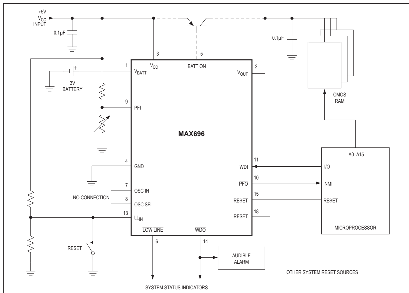
Figure 1. MAX696 Typical Application
