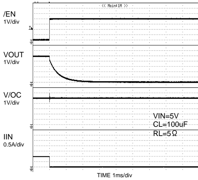
Figure 31. Output fall characteristics
