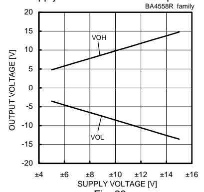
Fig. 28 Maximum Output Voltage - Supply Voltage (RL=2[kΩ], Ta=25[°C])
