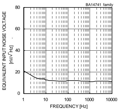
Fig. 239 Equivalent Input Noise Voltage - Frequency ( V_{CC}/V_{EE}=+15[V]/-15[V] , R_s=100[\Omega] , T_a=25[°C] )
