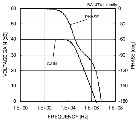
Fig. 242 Voltage Gain - Frequency ( V_{CC}/V_{EE}=+15[V]/-15[V] , A_v=40[dB] , R_L=2[k\Omega] , T_a=25[°C] )
