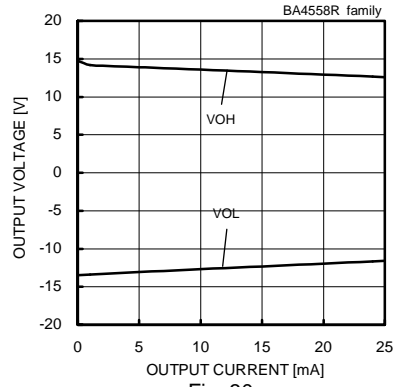
Fig. 30 Maximum Output Voltage - Output Current
