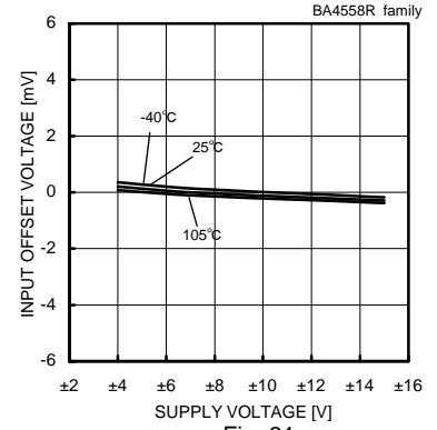
Fig. 31 Input Offset Voltage - Supply Voltage
