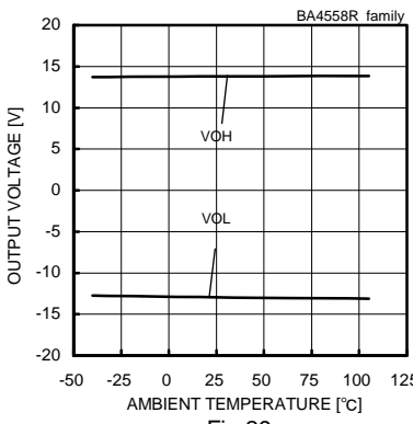
Fig. 29 Maximum Output Voltage - Ambient Temperature
