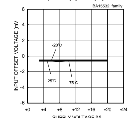
Fig. 251 Input Offset Voltage - Supply Voltage (Vicm=0[V], Vout=0[V])
