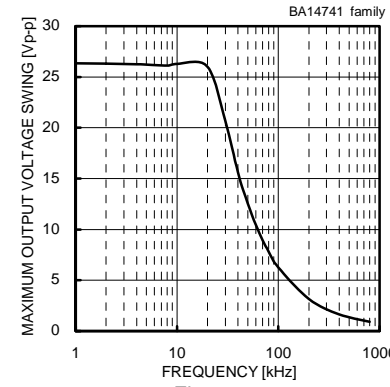
Fig. 241 Maximum Output Voltage Swing - Frequency ( V_{CC}/V_{EE}=+15[V]/-15[V] , R_L=2[k\Omega] , T_a=25[°C] )
