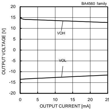
Fig. 52 Maximum Output Voltage - Output Current (VCC/VEE=+15[V]/-15[V], Ta=25[°C])
