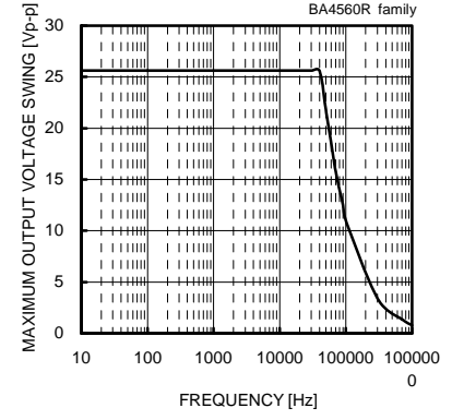
Fig. 87 Maximum Output Voltage Swing - Frequency (VCC/VEE=+15[V]/-15[V], RL=2[kΩ], Ta=25[°C])
