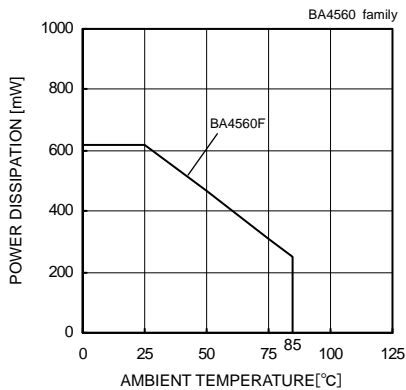
Fig. 45 Derating Curve
