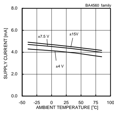
Fig. 47 Supply Current - Ambient Temperature
