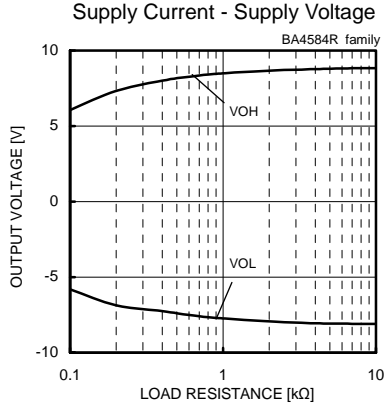
Fig. 159 Maximum Output Voltage - Load Resistance (VCC/VEE=+9.5[V]/-9.5[V], Ta=25[°C])
