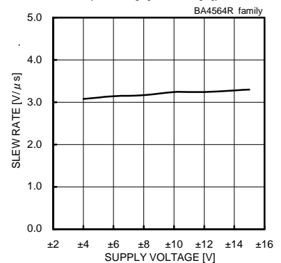
Fig. 106 Slew Rate - Supply Voltage ( C_L=100[pF] , R_L=2[kΩ] , T_a=25[°C] )
