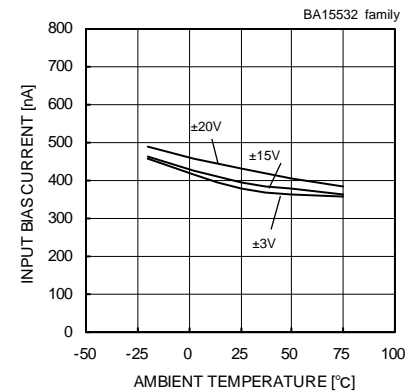
Fig. 254 Input Bias Current - Ambient Temperature (Vicm=0[V], Vout=0[V])
