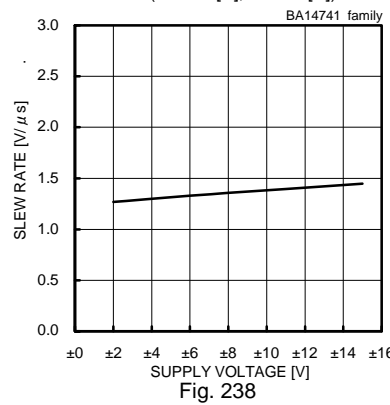
Fig. 238 Slew Rate - Supply Voltage ( C_L=100[pF] , R_L=2[kΩ] , T_a=25[°C] )
