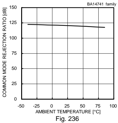
Fig. 236 Common Mode Rejection Ratio - Ambient Temperature ( V_{CC}/V_{EE}=+15[V]/-15[V] , V_{icm}=-12[V] to +12[V] )
