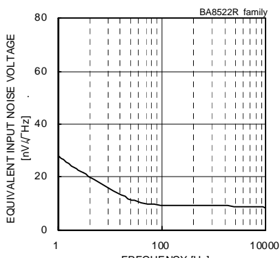
Fig. 195 Equivalent Input Noise Voltage - Frequency (VCC/VEE=+15[V]/-15[V], Rs=100[Ω], Ta=25[°C])
