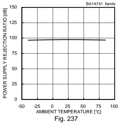
Fig. 237 Power Supply Rejection Ratio - Ambient Temperature ( V_{CC}/V_{EE}=+2[V]/-2[V] to +15[V]/-15[V] )
