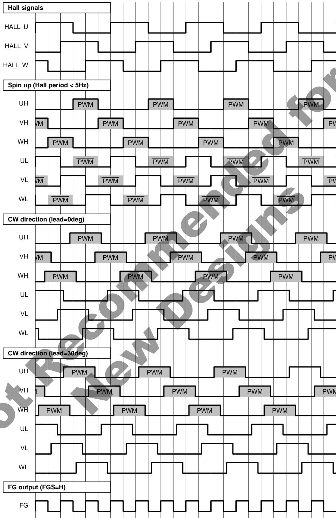
Figure 7. BD62012FS (Clockwise) timing charts
