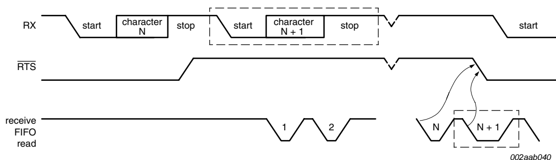
(1) N = receiver FIFO trigger level. (2) The two blocks in dashed lines cover the case where an additional character is sent, as described in Section 7.2.1
