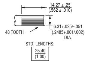
SHAFT TYPE "W" (USES BUSHING A)
