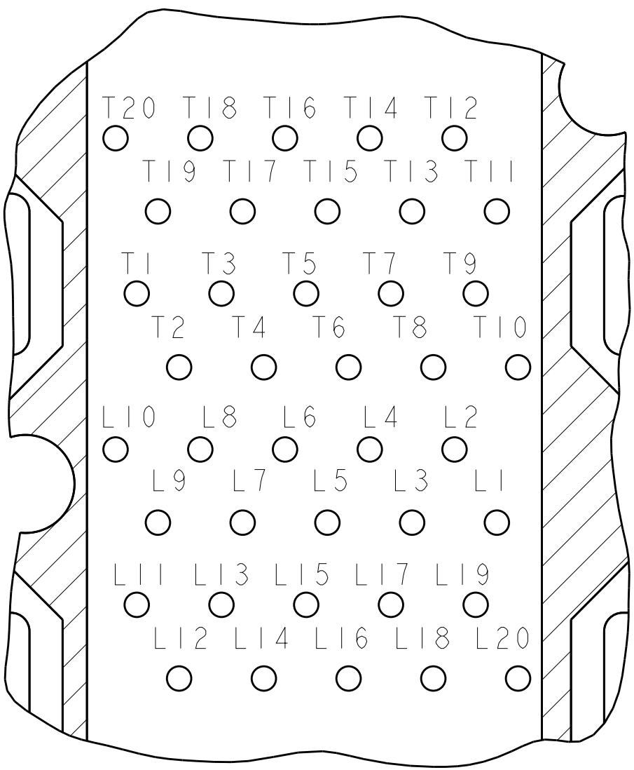
DETAIL H CONNECTOR PIN-OUT COMPONENT SIDE OF BOARD SCALE 10:1
