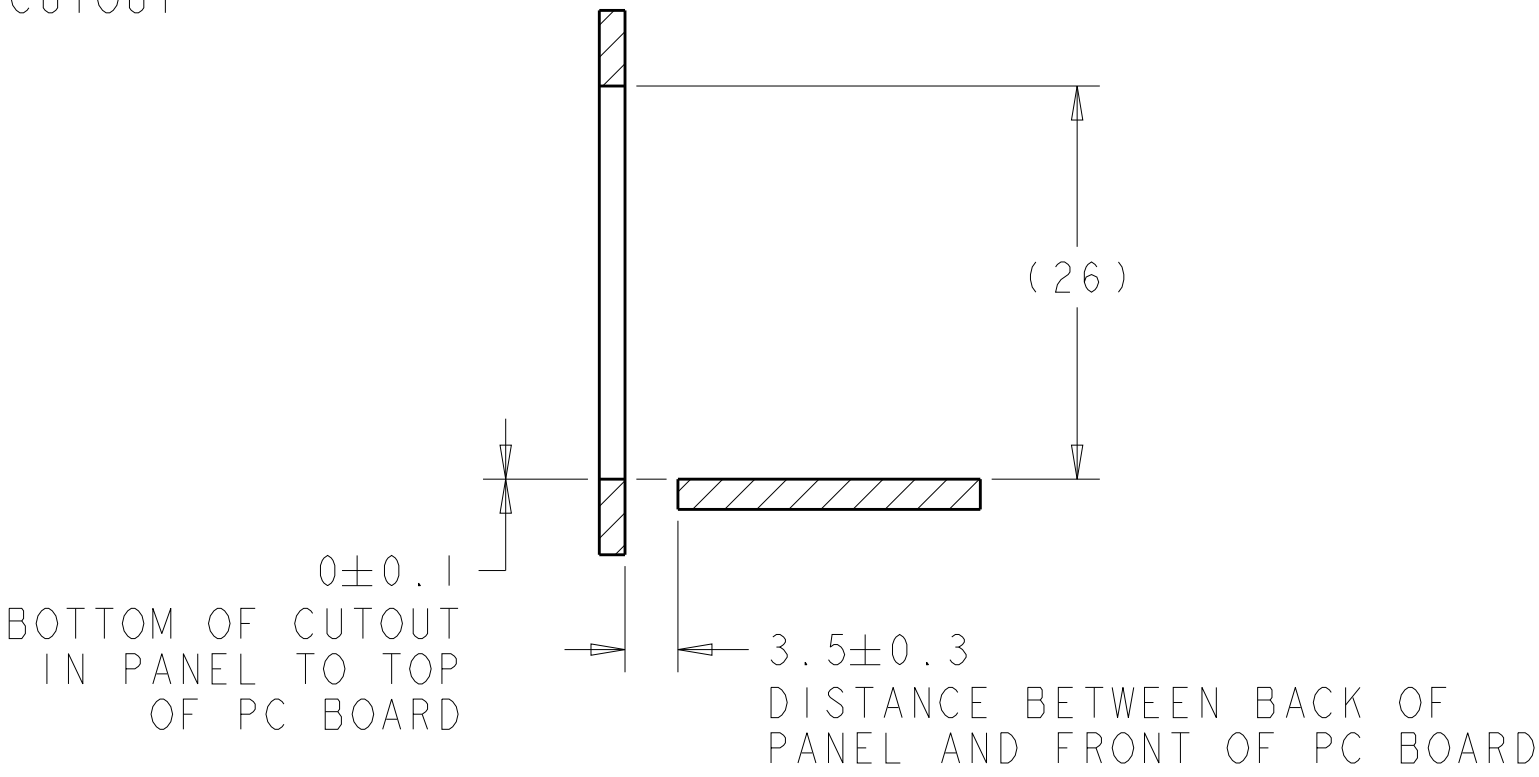
SECTION U-U
