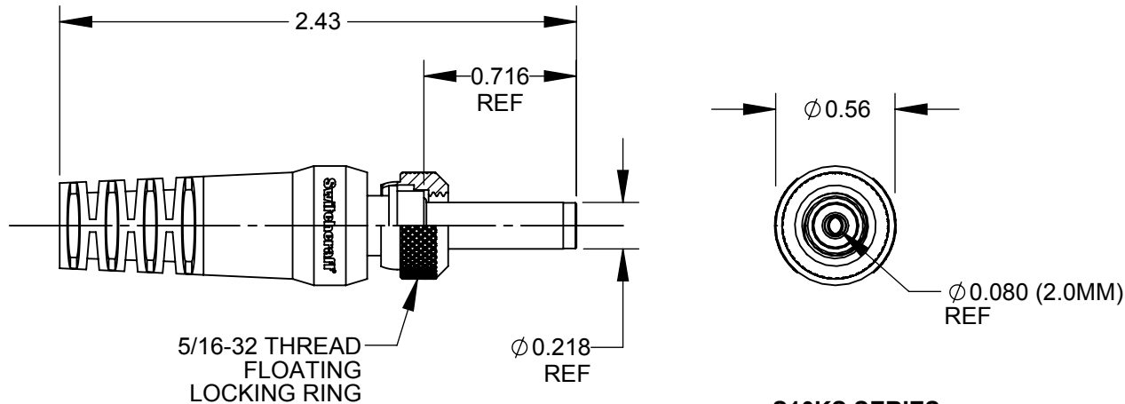
S10KS SERIES SEALED HI-AMP PLUG
