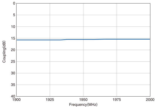
COUPLING
