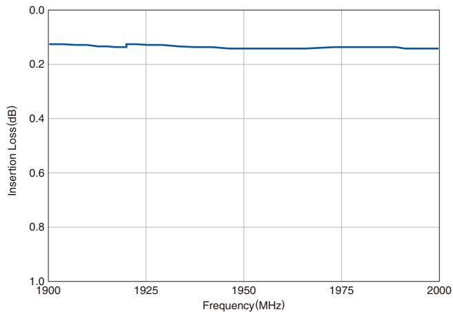
INSERTION LOSS
