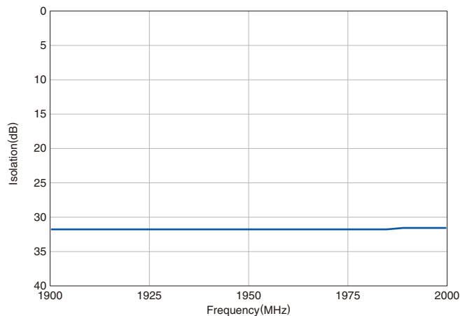
ISOLATION
