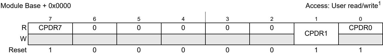
Figure 17-2. Port CP Data Register (CPDR)
