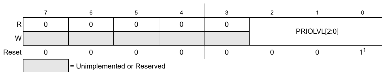
Figure 5-10. Interrupt Request Configuration Data Register 5 (INT_CFDATA5)
