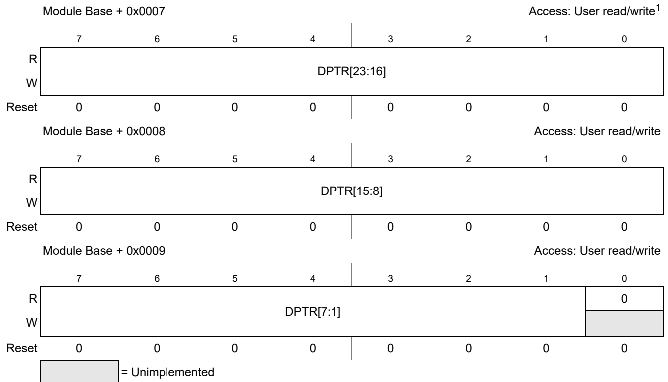
Figure 7-5. ECC Debug Pointer Register (ECDDPTRH, ECDDPTRM, ECDDPTRL)
