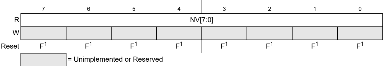
Figure 22-16. Flash Option Register (FOPT)
