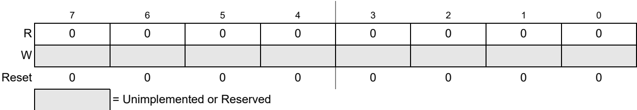
Figure 22-17. Flash Reserved1 Register (FRSV1)
