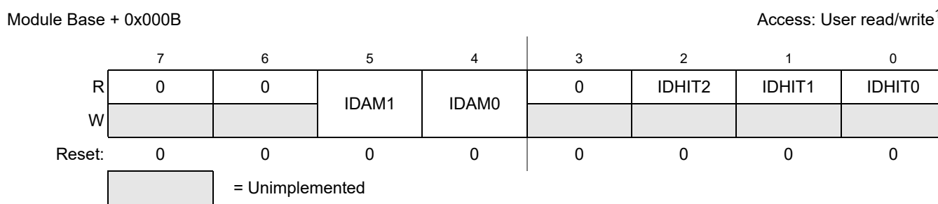
Figure 18-15. MSCAN Identifier Acceptance Control Register (CANIDAC)
