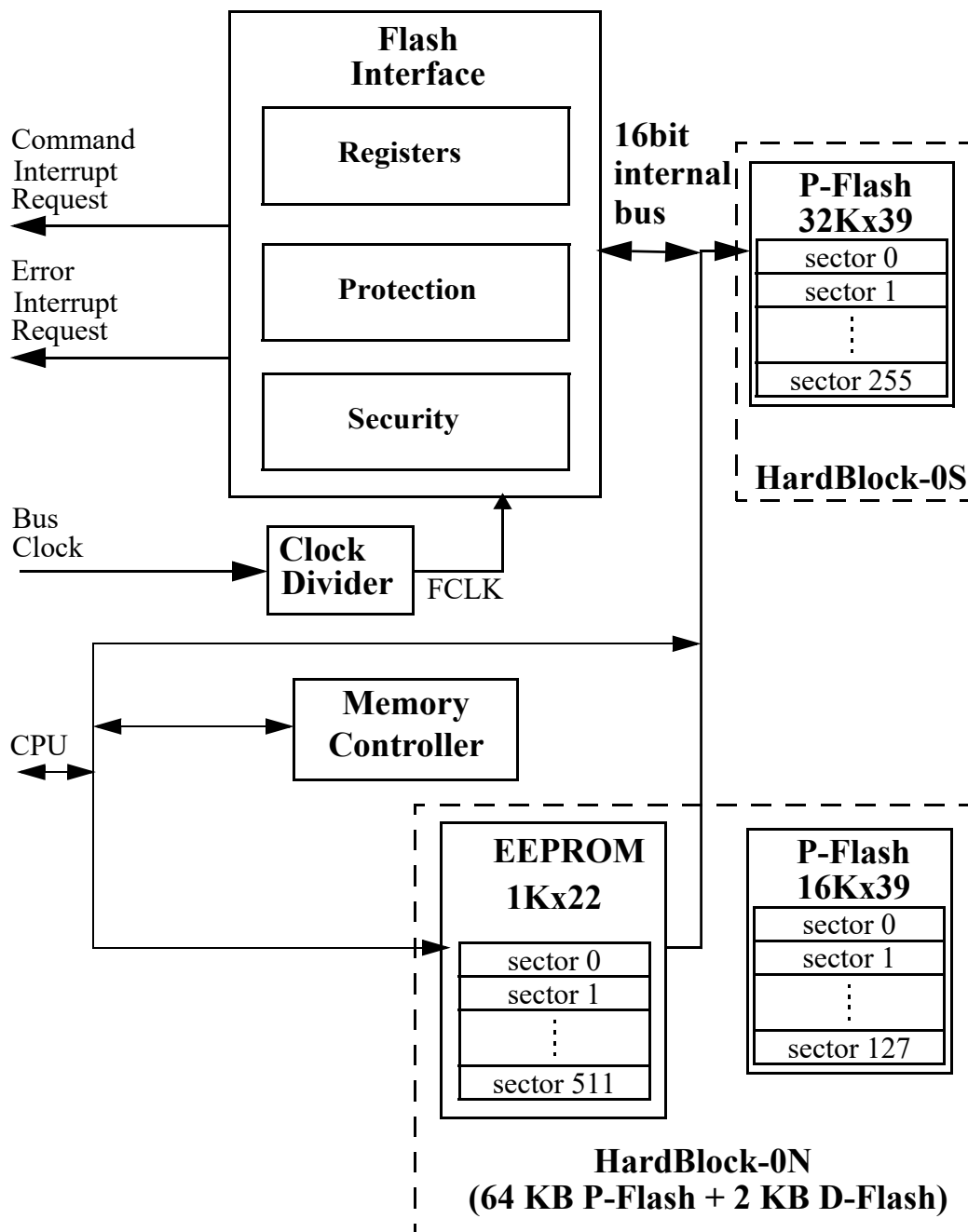
Figure 22-1. FTMZ192K2K Block Diagram
