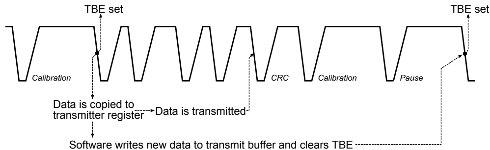
Figure 21-5. Transmit-Buffer Empty driven SENT transfer with Pause Pulse
