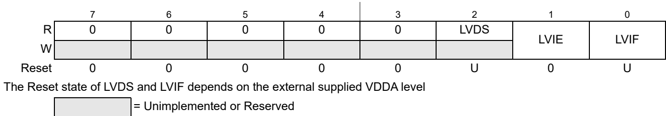
Figure 8-19. Low Voltage Control Register (CPMULVCTL)
