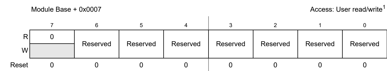
Figure 19-5. Reserved Registerfv_dac_8b5v_RESERVED
