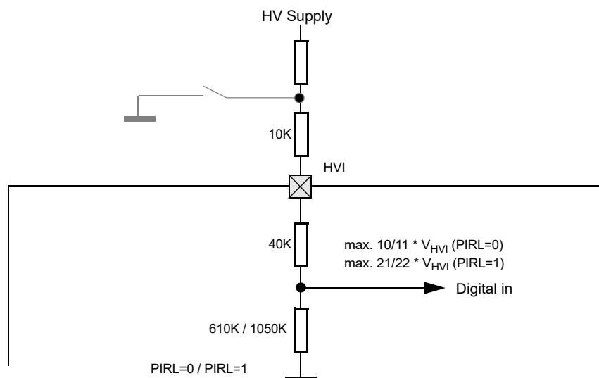
Figure 2-37. Digital Input Read with Pulldown Enabled
