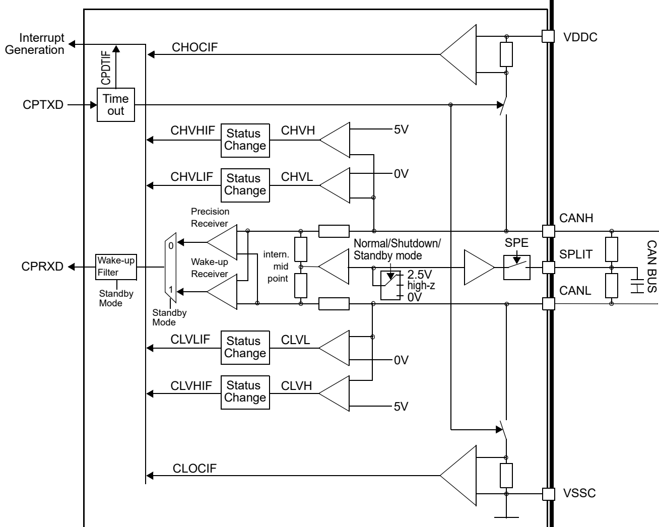
Figure 17-1. CAN Physical Layer Block Diagram
