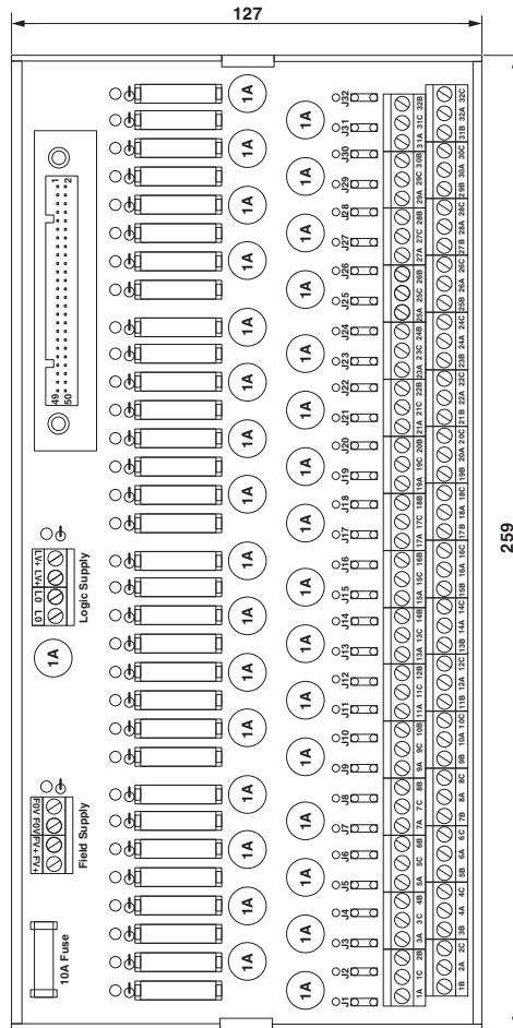
Dimensional drawing
