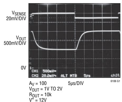
Step Response 10mV to 20mV ( R_{IN} = 100\Omega )
