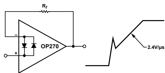
Figure 40. Pulsed Operation
