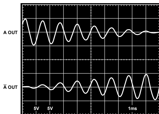
Figure 45. Digital Panning Control Output
