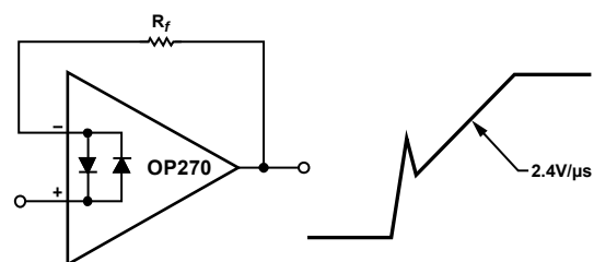
Figure 40. Pulsed Operation
