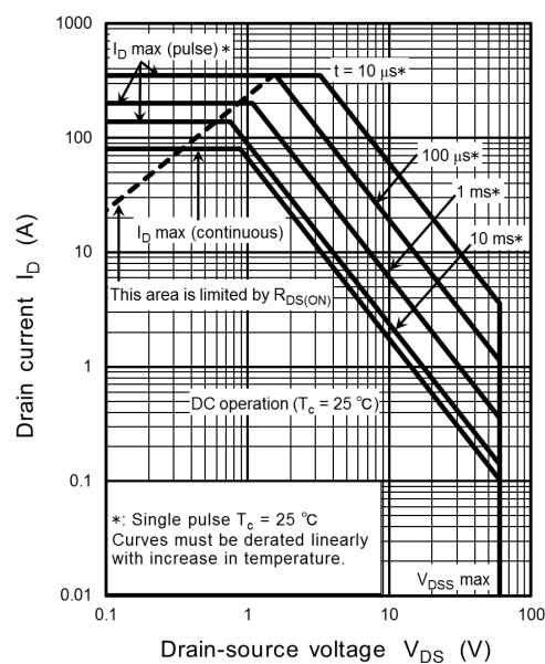
Fig. 8.15 Safe Operating Area (Guaranteed Maximum)
