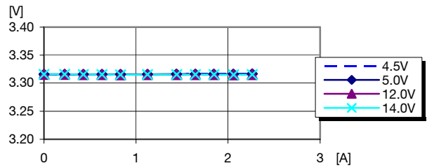
Output voltage vs. load current at T_{ref} = +25^{\circ}C
