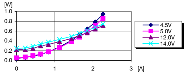
Dissipated power vs. load current and input voltage at T_{ref} = +25^{\circ}C
