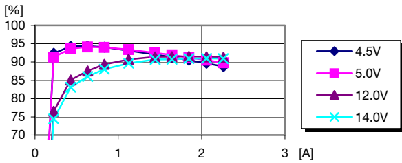
Efficiency vs. load current and input voltage at T_{ref} = +25^{\circ}C
