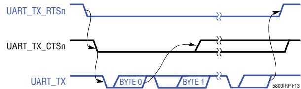
Figure 13. UART Mode 2 Transmit Flow Control
