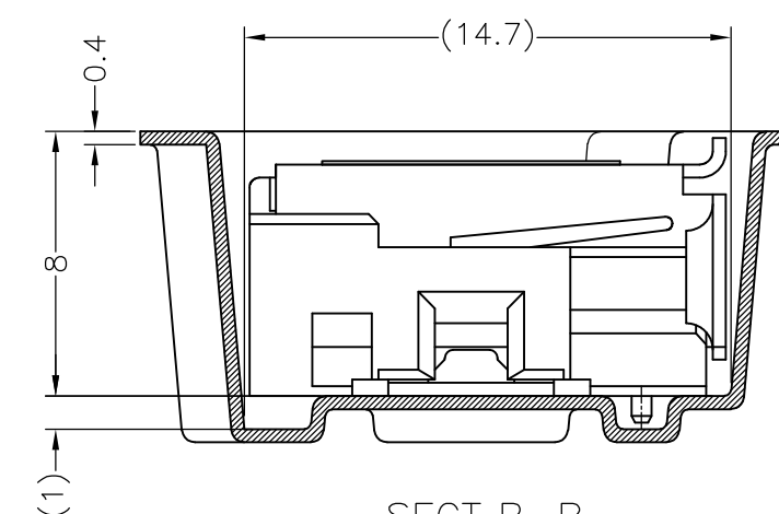
SECT B-B (4:1)
