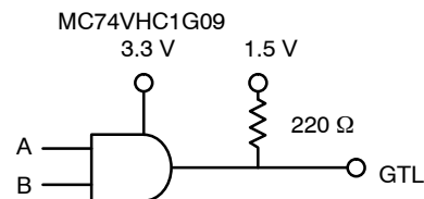
Figure 9. GTL Driver
