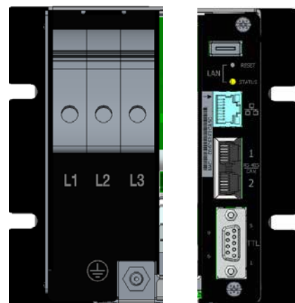
Input and Comms Standard Markings (View of 24KW shown. Comms interface is horizontal on the 12KW). See mechanical drawings.
