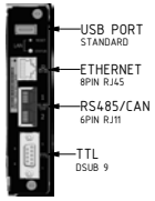
COMMS CONNECTORS DETAIL VIEW ROTATED 90° SCALE 1:2
