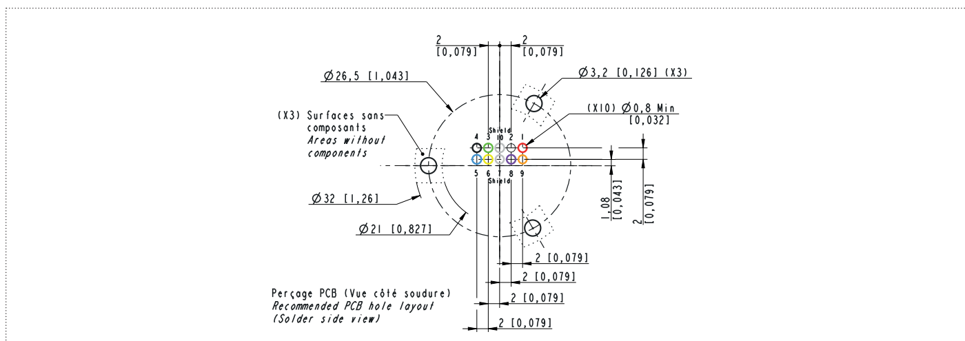
PCB Layout
