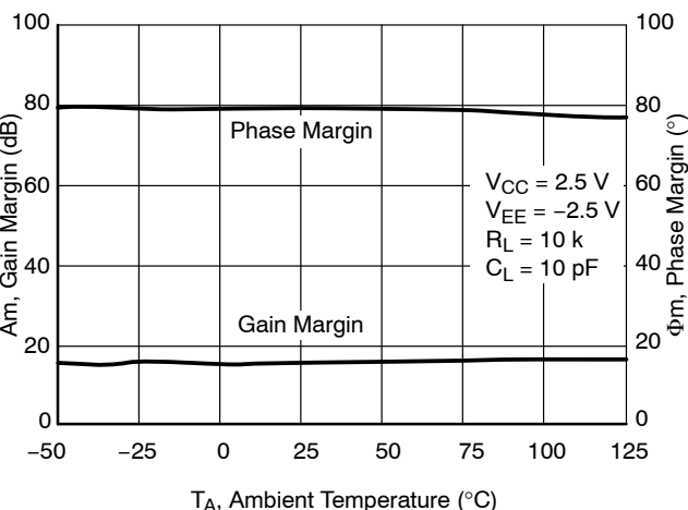
Figure 21. Gain and Phase Margin vs. Temperature
