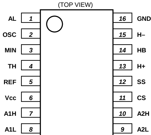
Fig.1 Pin configuration
