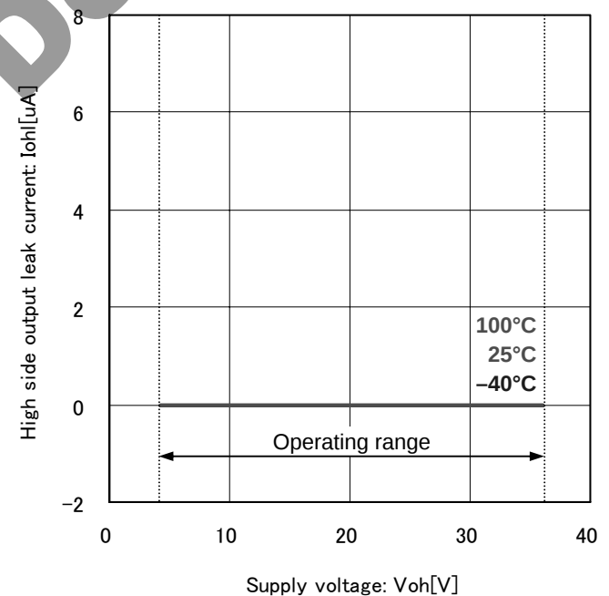
Fig.6 High side output leak current
