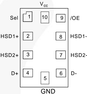
Figure 2. Pad Assignments for MicroPak™ (Top Through View)
