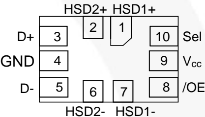
Figure 3. Pin Assignments for UMLP (Top Through View)
