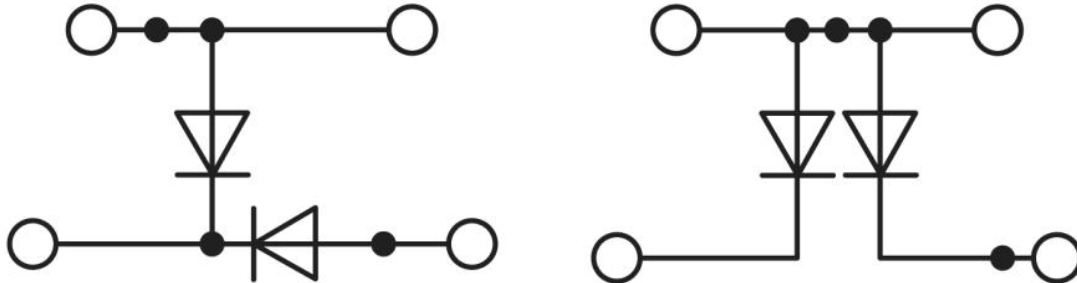
Circuit diagram
