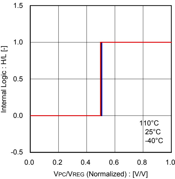
Figure 34. PWM Switching Arm Threshold Voltage
