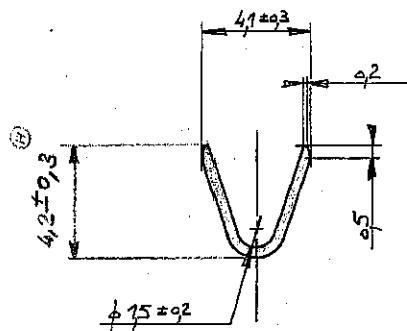
Section B
