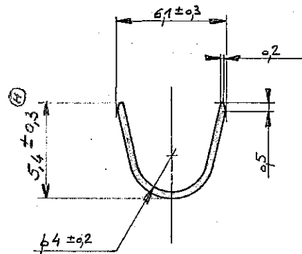
Section C
