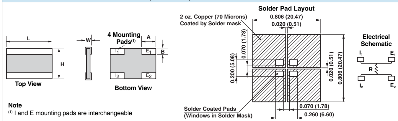
FIGURE 2 - DIMENSIONS in Inches (Millimeters)
