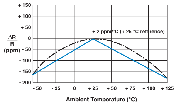
FIGURE 4 - TYPICAL RESISTANCE VERSUS TEMPERATURE CURVE AND ITS CHORD SLOPES (TCR)
