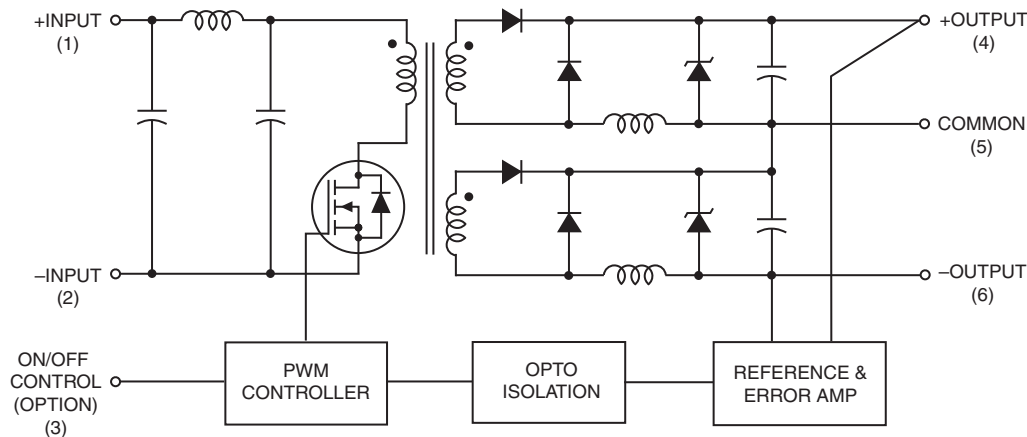
Figure 1. Simplified Schematic
