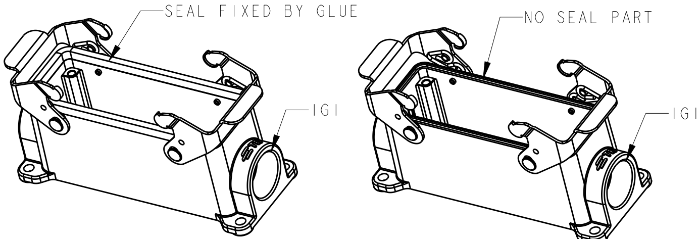
TYPE 4: BODY + STEEL LOCKING SIDE ENTRY OTHER SPEC REFER TO TYPE 3
