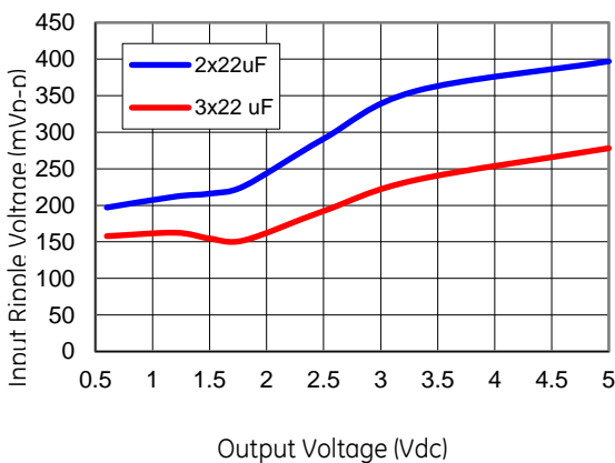
Figure 37. Input ripple voltage for various output voltages with 2x22 μF or 3x22 μF ceramic capacitors at the input (20A load). Input voltage is 12V.
