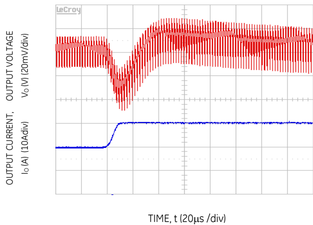
Figure 16. Transient Response to Dynamic Load Change from 50% to 100% at 12Vin, Cout= 2x47uF +3x330uF, CTune=5600pF & RTune=220 ohms
