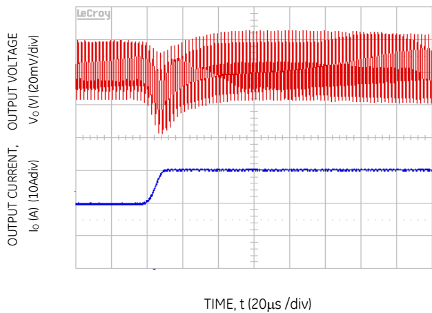
Figure 10. Transient Response to Dynamic Load Change from 50% to 100% at 12Vin, C_{out} = 1 \times 47 \mu F + 5 \times 330 \mu F , C_{Tune} = 10nF & R_{Tune} = 178 \text{ ohms}
