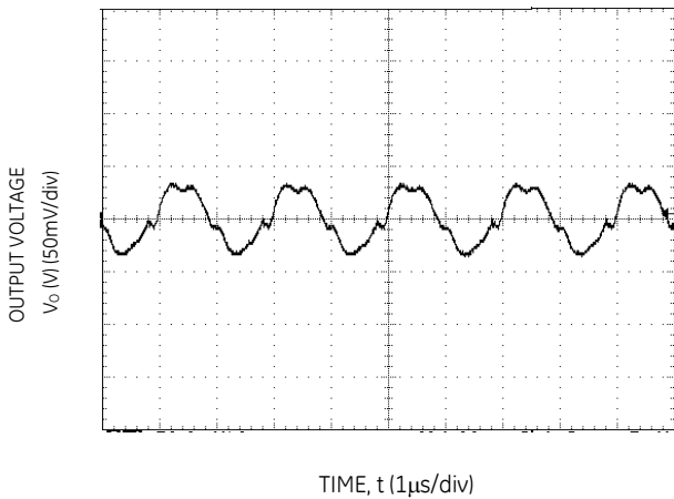
Figure 33. Typical output ripple and noise ( C_o=2 \times 47 \mu F ceramic, V_{IN} = 12V , I_o = I_{o,max} ).
