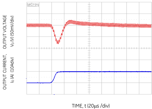
Figure 34. Transient Response to Dynamic Load Change from 50% to 100% at 12Vin, C_{out}= 8 \times 47 \mu F , C_{Tune}=1500 pF & R_{Tune}=220 \text{ ohms}
