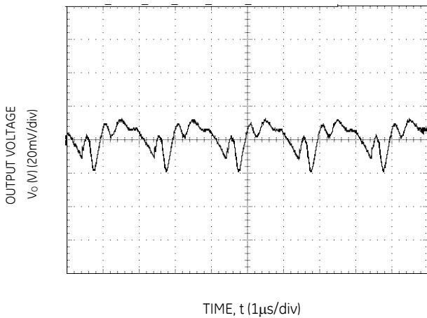
Figure 9. Typical output ripple and noise (C o =2x47μF ceramic, V IN = 12V, I o = I o,max ).
