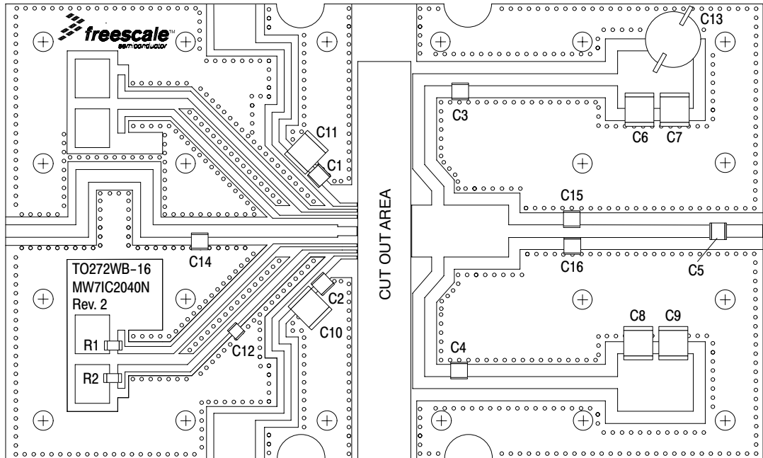
Figure 19. MW7IC2040NR1(GNR1)(NBR1) Test Circuit Component Layout — 1805-1880 MHz
