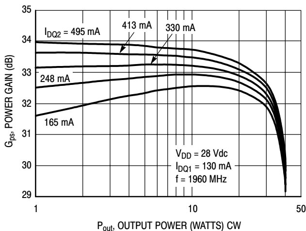
Figure 6. Power Gain versus Output Power @ I_{DQ1} = 130 \text{ mA}
