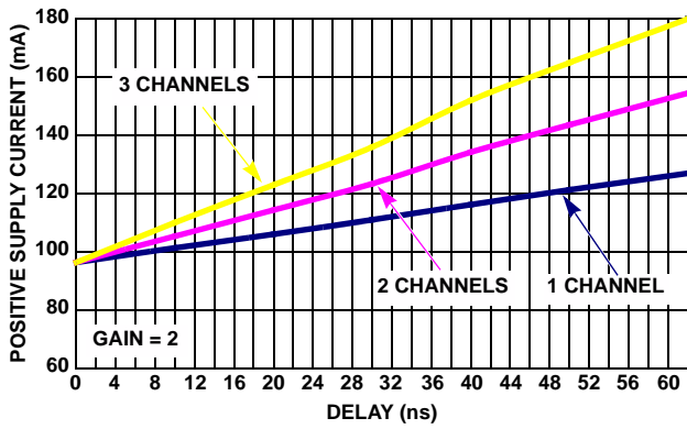
FIGURE 21. ISL59920 POSITIVE SUPPLY CURRENT ( V_{SP} ) vs DELAY TIME
