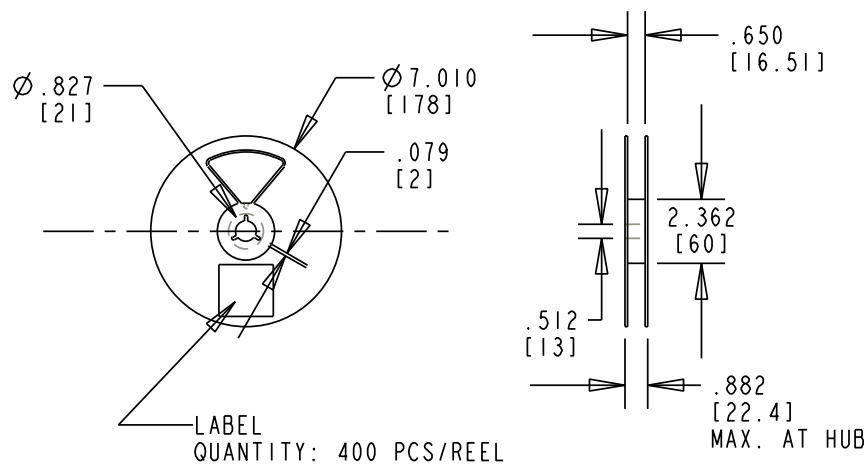
7 INCH DIA. REEL SPECIFICATIONS
