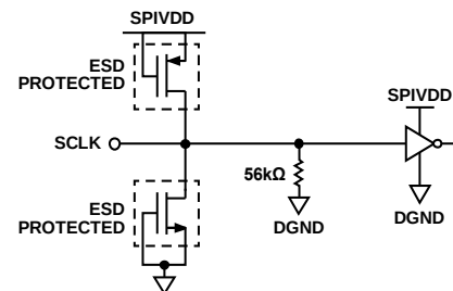
Figure 62. SCLK Input
