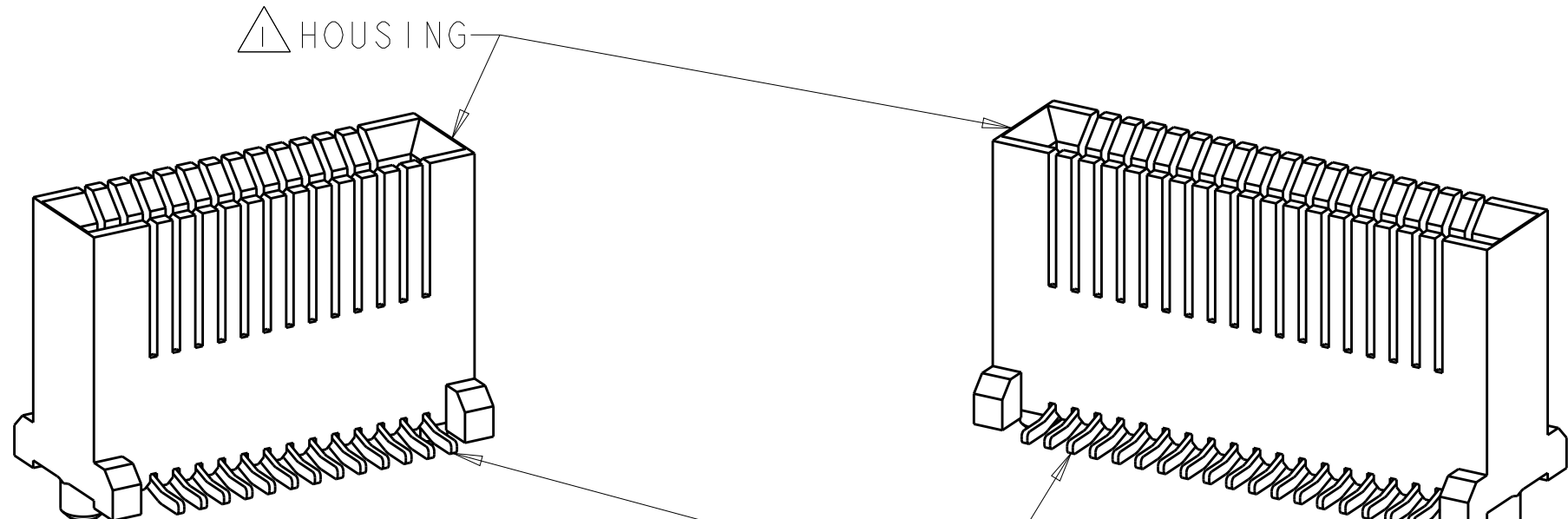
1888020-1 & -5 SCALE 5:1
