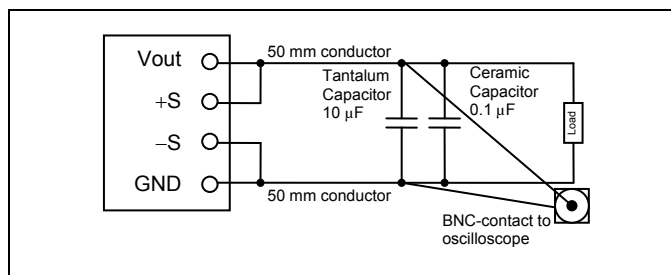
Output ripple and noise test set-up.
