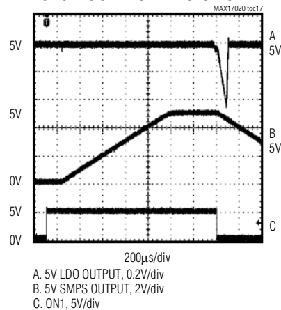
5V SMPS STARTUP AND SHUTDOWN
